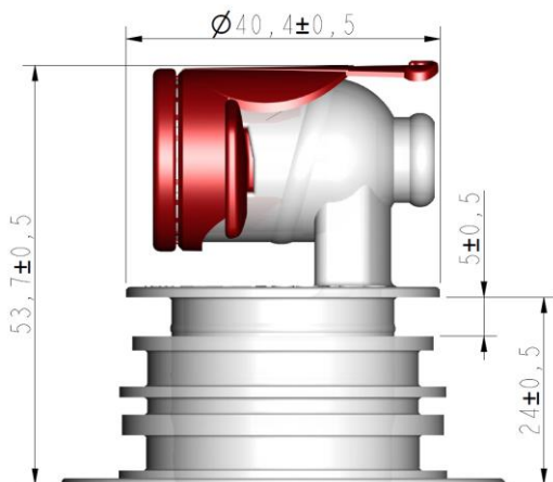
Vitop Standard tap inserted to pre-assembled position with the Vitop Aseptic Spout.
