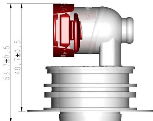
Vitop Uno Standard tap inserted to assembled (final) position with the Vitop Aseptic Spout.
