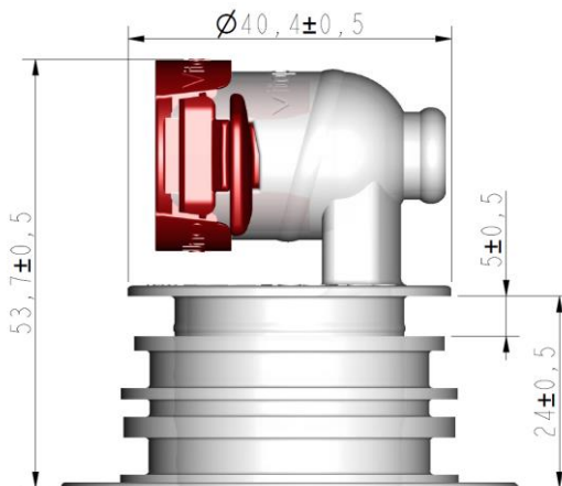
Vitop Uno Standard tap inserted to pre-assembled position with the Vitop Aseptic Spout.
