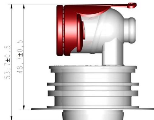
Vitop Standard tap inserted to assembled (final) position with the Vitop Aseptic Spout.
