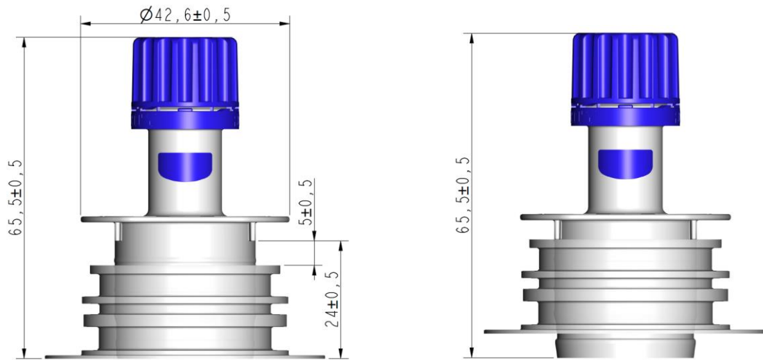
Vitop T-tap inserted to pre-assembled position with the Vitop Aseptic Spout.
